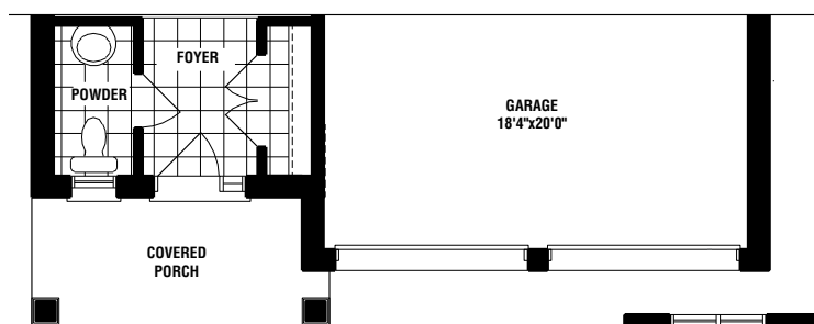
PART. GROUND FLOOR ELEV. 'B' & 'C'
