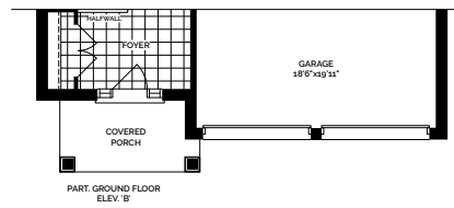
PART GROUND FLOOR ELEV. 'B'
